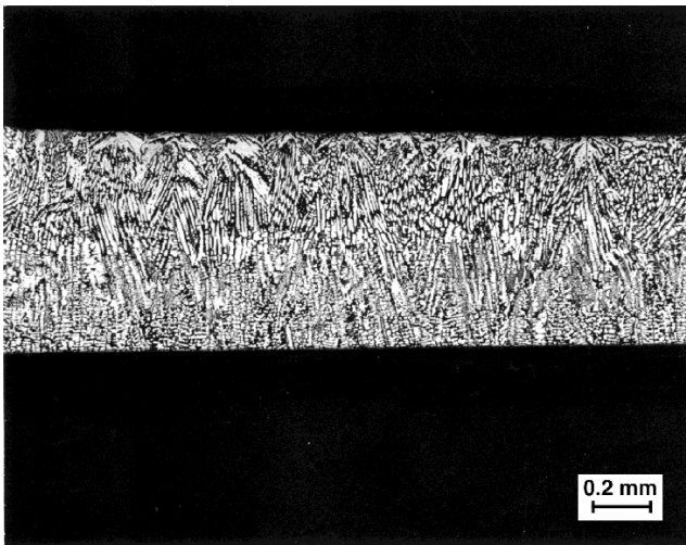
Fig. 11. Transverse solidification structure of a sample solidified on a textured substrate surface [200 \mu\text{m} ridge pitch]
