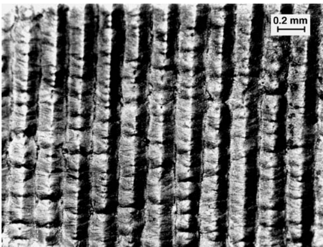
Fig. 8. Surface solidification structure of a sample solidified on a textured substrate surface [200 \mu\text{m} ridge pitch].
