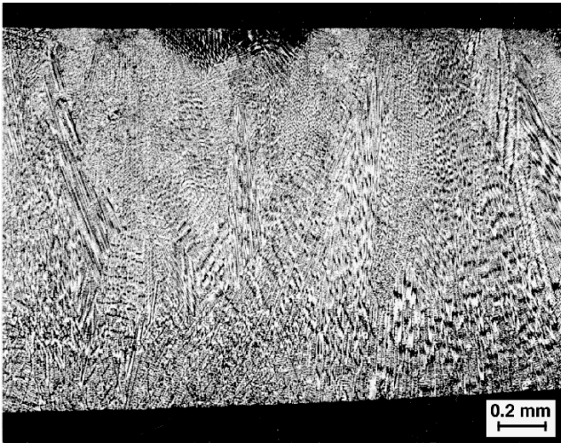
Fig. 10. Transverse solidification structure of a sample solidified on the smooth substrate surface.
