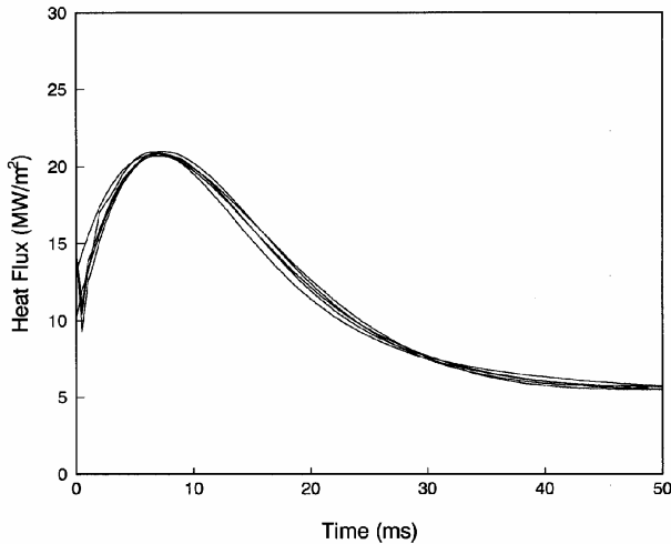
Fig. 3. Reproducibility of heat flux data from five consecutive immersions; textured substrate [150x30 \mu m], 75 degrees melt superheat, 0.5m/s immersion velocity, argon atmosphere.
