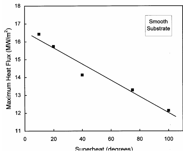
Fig. 15. The effect of melt superheat on the maximum heat flux.
