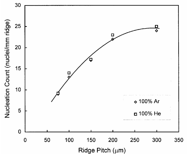
Fig. 13. The effect of substrate surface textures on the nucleation count along the ridges for samples solidified using argon and helium gas atmospheres.
