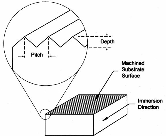
Fig. 4. Schematic of substrate surface texture showing machined ridges parallel to the immersion direction.
