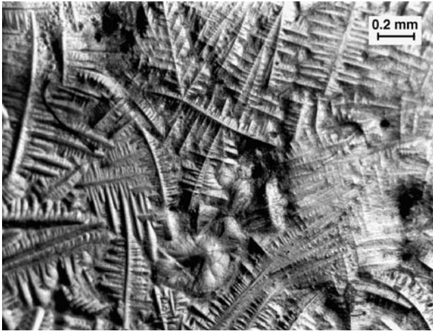
Fig. 7. Surface solidification structure of a sample solidified on the smooth substrate surface.
