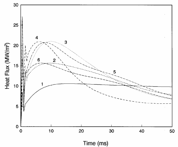
Fig. 5. Heat flux histories for samples solidified on various substrate surfaces; texture details given in Table 2.
